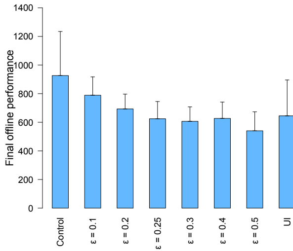
Fig. 12 Final offline learning performance for different \epsilon values and original Control and UI conditions. Note that error bars stand for standard error of the mean.
