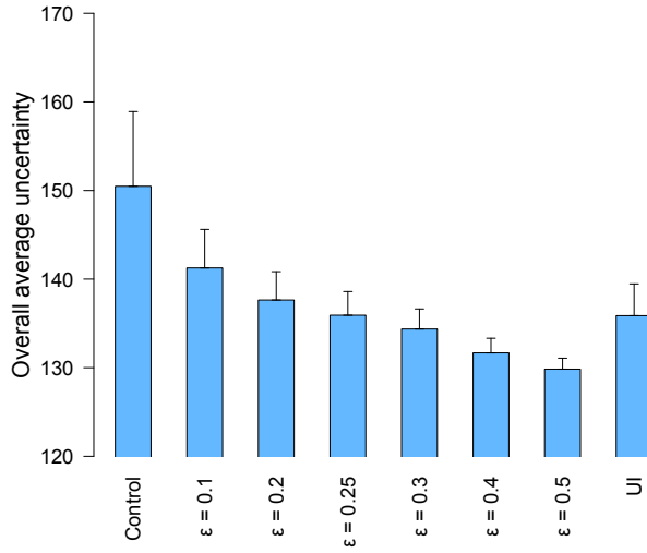
Fig. 11 Overall average uncertainty across subjects for different \epsilon values and original Control and UI conditions. Note: error bars stand for standard error of the mean.
