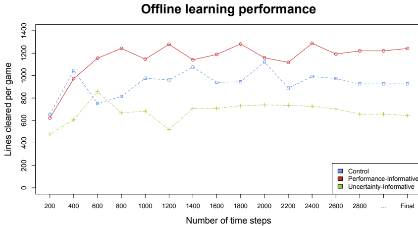
Fig. 7 Offline performance per cumulative 200 time steps for the three conditions. Control condition: blue (middle), performance-informative condition: red (top), uncertainty-informative condition: green (bottom).
