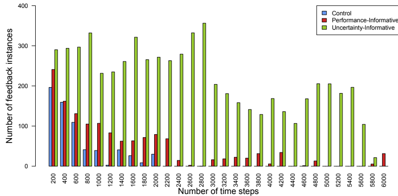
Fig. 6 Number of feedback instances per 200 time steps over the first 6000 time steps. Control condition: blue (left), performance-informative condition: red (middle), uncertainty-informative condition: green (right).
