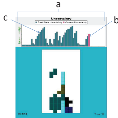
Fig. 2 The uncertainty-informative interface: (a) the uncertainty graph window, (b) the current uncertainty (pink bar), and (c) the uncertainty of past actions (dark blue bar).
