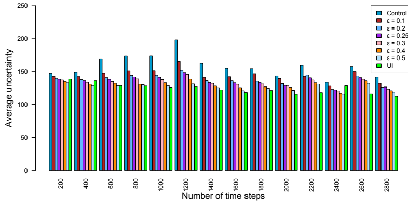
Fig. 13 Average uncertainty per 200 time steps across subjects during the training process for different \epsilon values and original Control and UI conditions. Note: from left to right, each bar represents the corresponding value for the original Control condition, \epsilon = 0.1 , \epsilon = 0.2 , \epsilon = 0.25 , \epsilon = 0.3 , \epsilon = 0.4 , \epsilon = 0.5 and the original UI condition, respectively.
