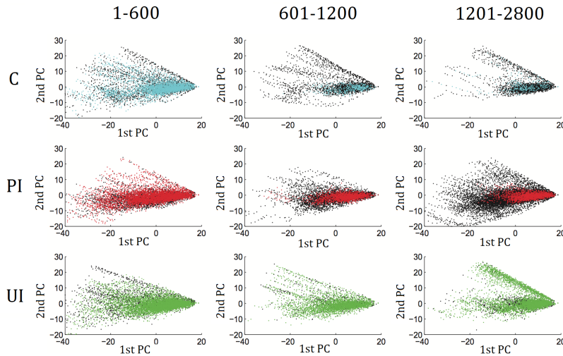
Fig. 8 Distribution of states along the first (horizontal axis) and second (vertical axis) principal components (PC), with (colored according to corresponding conditions) and without (colored black) feedback. The three rows from top to bottom show the control (C), performance-informative (PI) and uncertainty-informative (UI) conditions respectively. The columns show three sections of the training process: time steps 1-600, 601-1200, and 1201-2800, from left to right, respectively. Note that these graphs were generated by first plotting the states without feedback and then overlaying the colored states where feedback was received.
