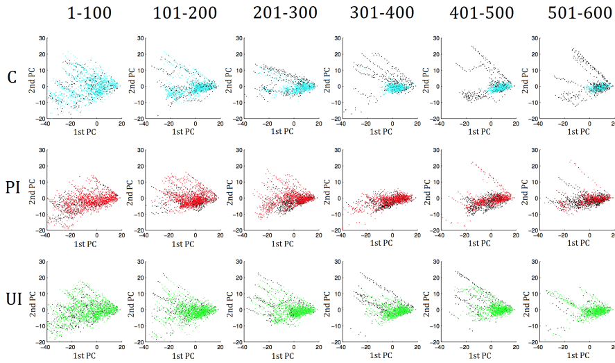
Fig. 10 More detailed visualisation of the data from the first column of Figure 8 at a finer temporal resolution. Distribution of states along the first (horizontal axis) and second (vertical axis) principal components (PC), with (colored according to corresponding conditions) and without (colored black) feedback for the first 600 time steps during the training process. The three rows from top to bottom show the control (C), performance-informative (PI) and uncertainty-informative (UI) conditions respectively. The columns show time steps 1-100, 101-200, 201-300, 301-400, 401-500 and 501-600, from left to right, respectively.
