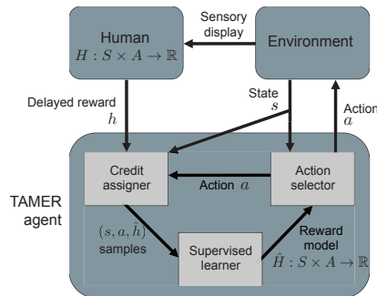
Fig. 1 Interaction in the TAMER framework (reproduced from [17]).
