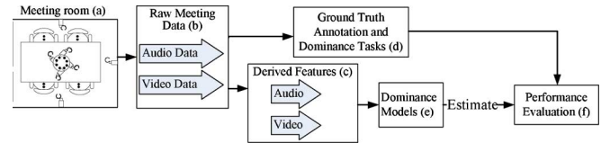
Fig. 1. Flow diagram of our approach.
