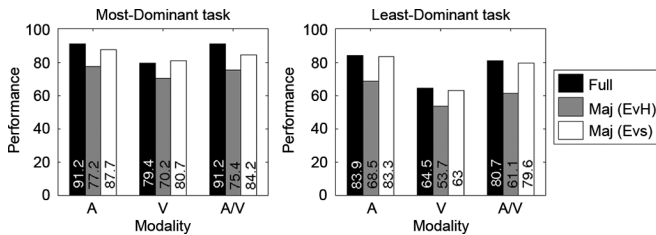
Fig. 7. Comparison of the best performance values in each modality and each dominance sub-task. A: Audio, V: Video, A.V: Audio-Visual.
