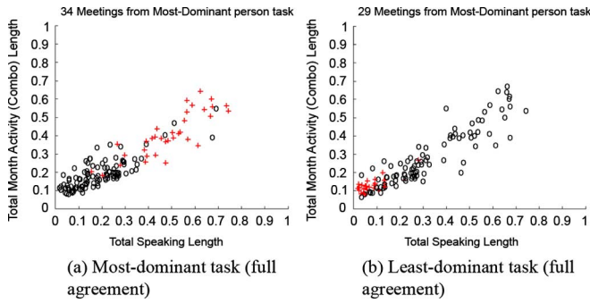
Fig. 6. Scatter plots of the total speaking length and visual activity length where the red crosses show the ground truth annotated person with the corresponding audio and visual cues, and the black circles show the negative class in each case.
